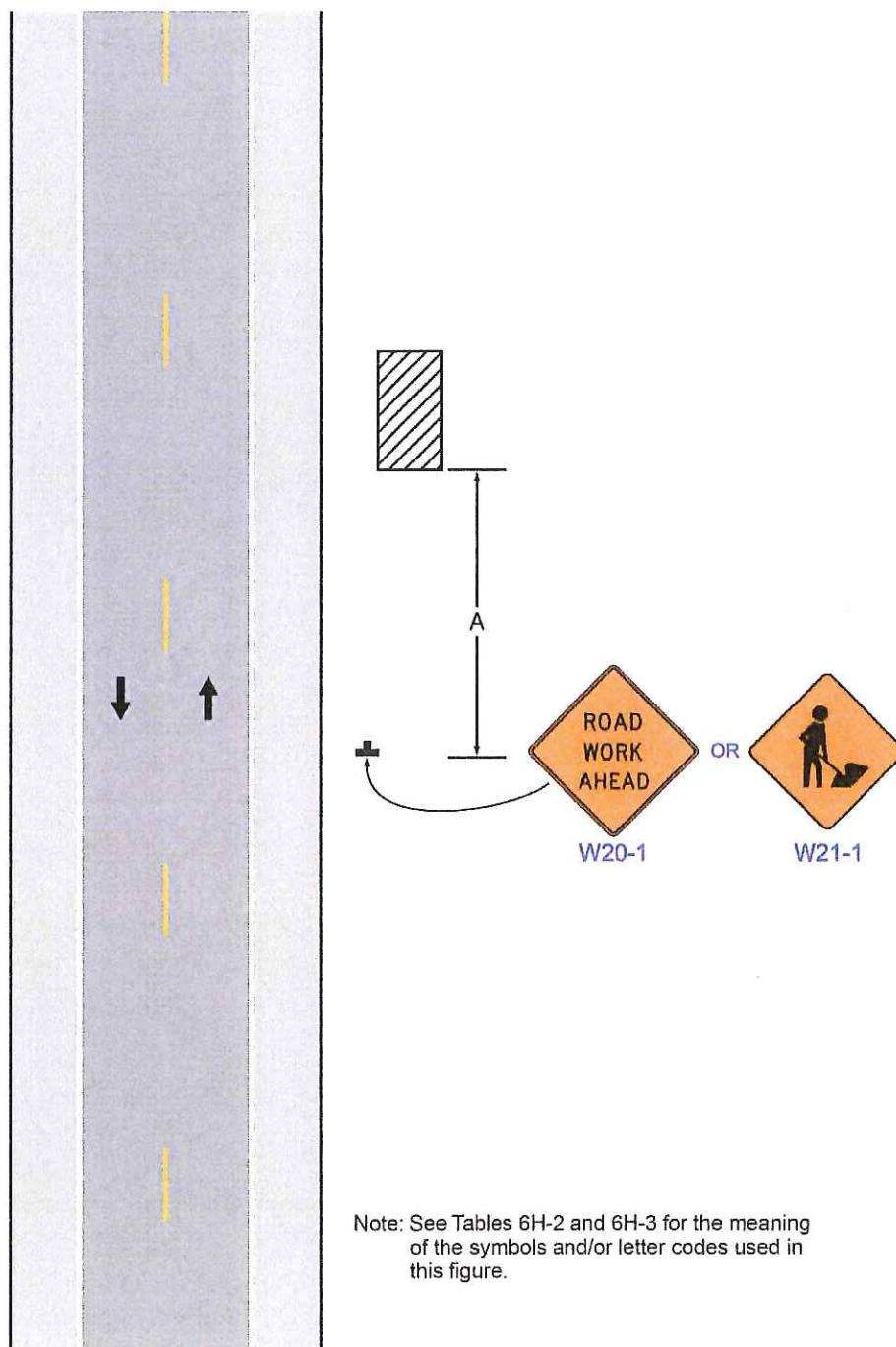
Typical Application 1
